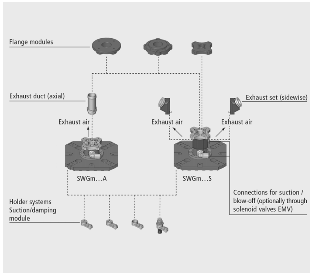
Exhaust duct ABL-FUEHR For controlled discharge of drawn-in air out of the process room (axial)
